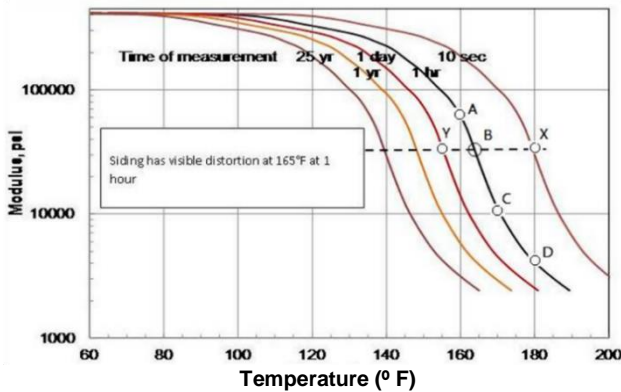
Figure 4. Vinyl Siding Modulus vs. Temperature with Respect to Time
