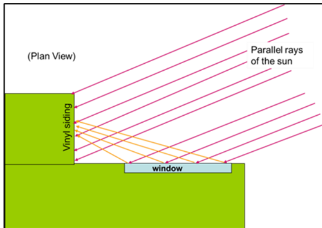
Figure 10. Inside Corner
