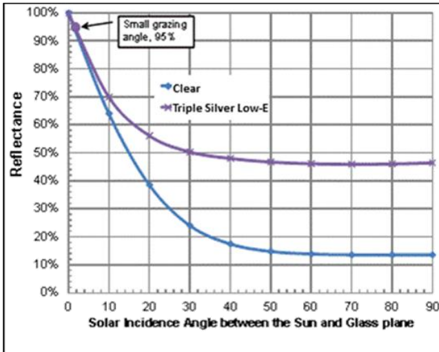
Figure 12. Reflectance at Grazing Angle
