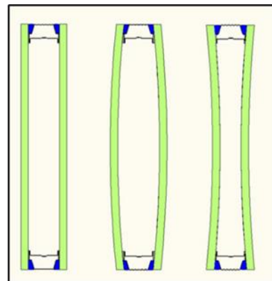
Figure 7. Dynamic Flexing
