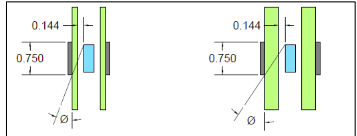
Figure IG08-1, In both cases: 0.522" airspace and 0.235 x 0.625" internal grille. Left utilizes 3mm (0.117") glass and right 8mm (0.296") glass.
