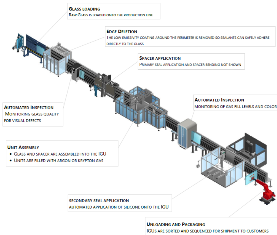
Figure 1: Flow diagram for Insulating Glass manufacturing steps
