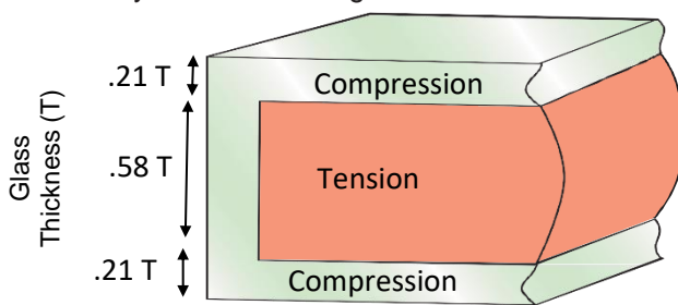
Fig. 6-1: Heat Strengthened Glass Compression and Tension Zones
