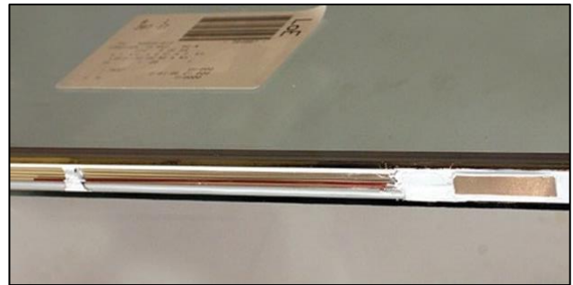
Fig 13-1: An installed capillary tube (colored red for photo only)
