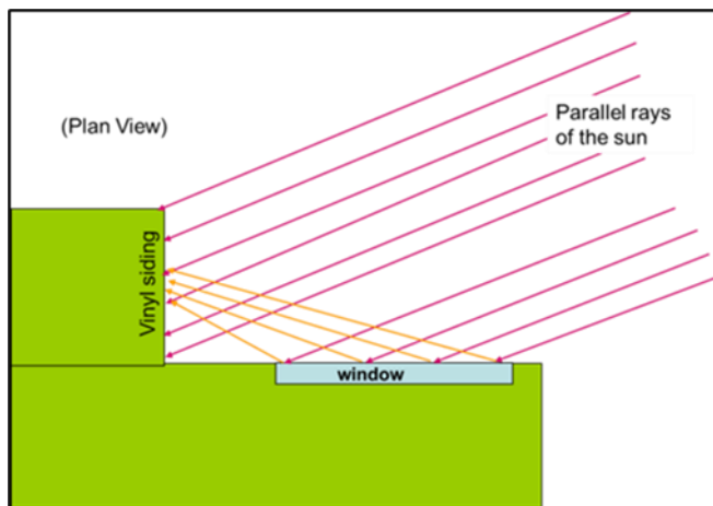
Figure 10. Inside Corner
